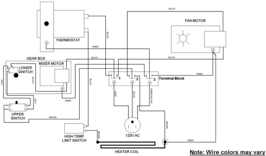
BioLet Deluxe Wiring Diagram
